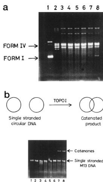
FIG. 3. a , relaxation of negatively and positively supercoiled DNA. 500 ng of negatively supercoiled DNA (Form I) (lane 1), was relaxed by 1 unit of M. smegmatis topoisomerase I in presence of 2 \mu g/ml ethidium bromide (lane 2). 1 \mu g of relaxed pUC19 DNA (Form IV) was used as substrate in lanes 3–8. All the assays mixtures contained 2 \mu g/ml ethidium bromide, with 1 and 2 units of E. coli (lanes 3 and 4), M. smegmatis (lanes 5 and 6), and calf thymus topoisomerase I (lanes 7 and 8), respectively. b , catenation assay with single-stranded M13 DNA. M13 single-stranded DNA (lane 1) was incubated with the assay buffer in absence of topoisomerase I at 52 °C (lane 2). The substrate was incubated with 2, 4, and 6 units of enzyme at 37 °C (lanes 3, 4, and 5) and at 52 °C (lanes 6, 7, and 8), respectively. The appearance of catenanes are indicated by arrow (lanes 7 and 8).
