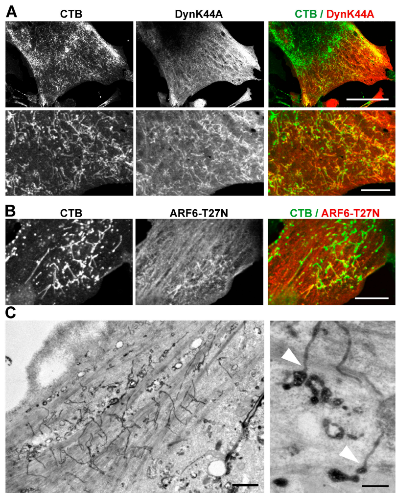
Figure 3. Dynamin and ARF6 mutants inhibit CTB transport to the Golgi complex. Cav1 -/- MEFs were microinjected with cDNA for DynK44A (A) or ARF6 T27N (B and C; short expression). CTB Alexa Fluor 594 was internalized for 40 min (A and B). DynK44A and ARF6 T27N that contained NH 2 -terminal HA tags were labeled with anti-HA (A and B). CTB colocalizes with DynK44A (A) and ARF6 T27N (B) in an extensive tubular network. This is highlighted in enlargements in bottom panels of A. (C) Cav1 -/- MEFs were microinjected with ARF6 T27N and HRP, and CTBHRP was internalized for 40 min at 37°C. Cells were prepared for EM and CTBHRP was revealed by DAB cytochemistry. CTBHRP reaction product was evident within a network of 40-nm-diam tubular structures in the injected cells, some of which connect to multivesicular regions (arrowheads). Bars: (A, top; and B) 25 μm; (A, bottom) 5 μm; (C, left) 1 μm; (C, right) 200 nm.
