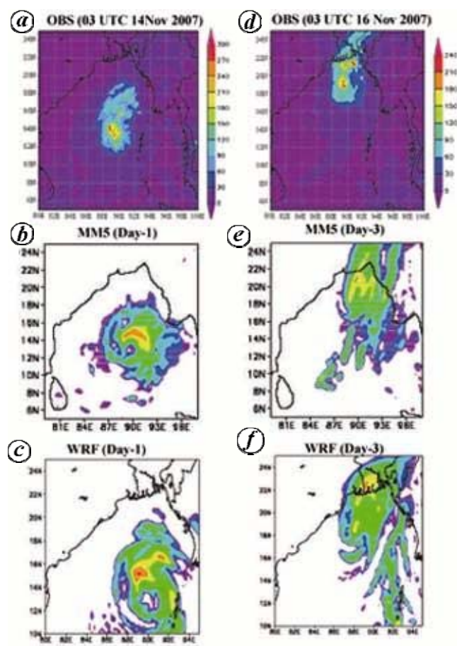
Figure 8. The 24 h accumulated precipitation for case-III (Sidr) from initial condition of 00 UTC 13 November 2007. a, Observed at 03 UTC 14 November 2007; b, Simulated with MM5 (day-1); c, simulated with WRF (day-1); d, Observed at 03 UTC 16 November 2007; e, Simulated with MM5 (day-3); and f, Simulated with WRF (day-3).
