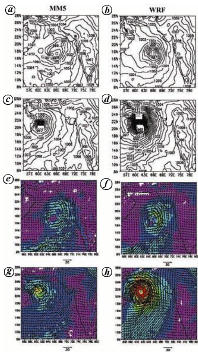
Figure 4. Simulation of MSLP and wind at 850 hPa for case-II (Gonu) from initial condition of 00 UTC 3 June 2007. a , MSLP for day-1 with MM5; b , MSLP for day-1 with WRF; c , MSLP for day-3 with MM5; d , MSLP for day-3 with WRF; e , Wind for day-1 with MM5; f , Wind for day-1 with WRF; g , Wind for day-3 with MM5, and h , Wind for day-3 with WRF.
