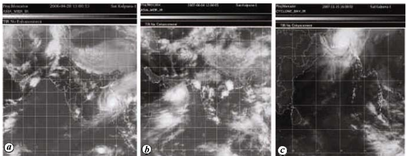
Figure 2. Satellite imagery as obtained from INSAT (Kalpana-1). Valid at (a) 13 UTC 28 April 2006 (Mala), (b) 12 UTC 4 June 2007 (Gonu) and (c) 16 UTC 15 November 2007 (Sidr).
