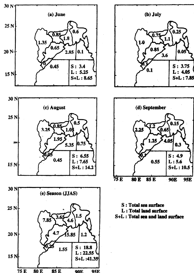
Figure 5. Mean frequency of LPS days over different regions during different monsoon months and the season.
