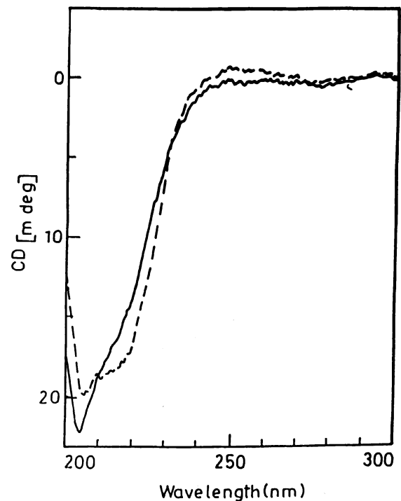
Fig. 3. CD spectra of ts2 mutant and wild-type repressors. The spectra were measured in 0.1 M potassium phosphate buffer, pH 8.0, at 25 ^{\circ} C. A protein concentration of 1 \mu M was used for both the repressors. Curves: solid line, ts2 repressor; broken line, wild-type repressor. For further details, see Materials and methods.
