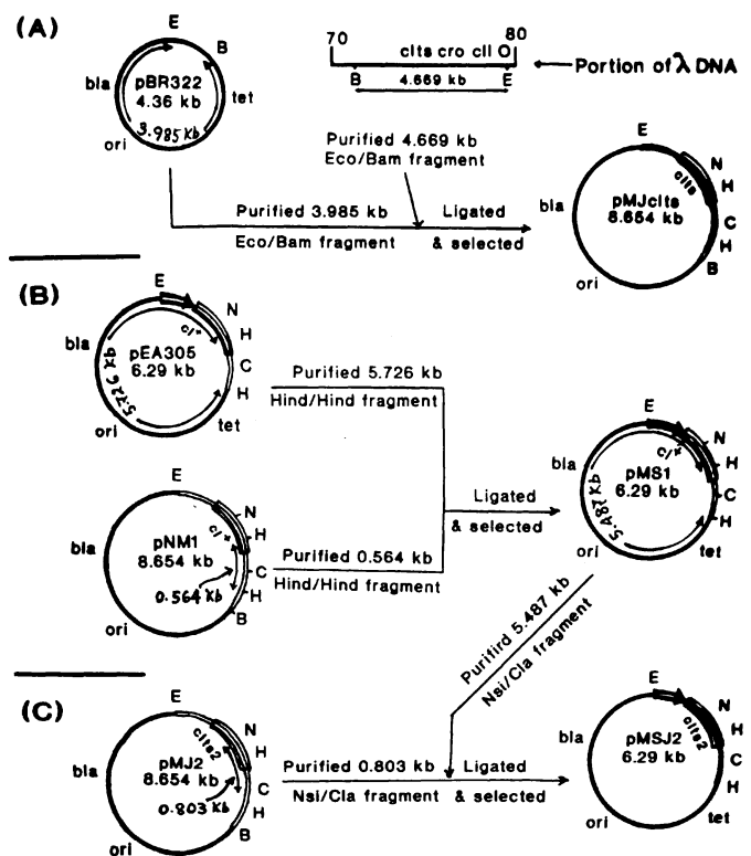
Fig. 1. Cloning of mutant cIts genes of \lambda . (A) The mutant cIts genes from \lambda cItsU50 , \lambda cItsU9 , \lambda cItsU46 , \lambda cIts1 , \lambda cItsU51 , \lambda cItsI-22 and \lambda cIts2 phages were cloned in pBR322 as shown. The constructed plasmid pMJcIts represents the general name for pMJ50, pMJ9, pMJ46, pMJ1, pMJ51, pMJ1-22 and pMJ2 for the clones of cIts genes, respectively, from the above cIts mutant phages. These plasmids were selected in E.coli DH5 by their immunity to superinfection by \lambda cI^- at 32°C and sensitivity to limm434cI^- at 32°C and \lambda cI^- at 42°C. Finally, each clone was confirmed by restriction analysis. (B) The plasmid pEA305 carries the wild-type cI gene of \lambda tagged to the tac promoter and expresses the repressor at very high level (around 30% of the total cellular protein) when induced by IPTG in a lacI H host (Amann et al. , 1983). This plasmid does not contain the Clal site between the C terminus of cI gene and the downstream HindIII site, whereas the plasmid pNM1 (Das and Mandal, 1986) carrying also the wild-type cI gene tagged to its P RM promoter has the Clal site at the analogous position. A cassette plasmid pMS1 carrying the cI + gene tagged to the tac promoter and containing the Clal site between C terminus and the downstream HindIII site was constructed by replacing the 0.564 kb HindIII/HindIII fragment of pEA305 by the same restriction fragment from pNM1. pMS1 was selected by testing its immunity to \lambda cI^- superinfection at both 32 and 42°C and detecting the presence of the Clal site, and by restriction analysis. (C) The plasmid pMSJ2 carrying the mutant cIts2 gene tagged to the tac promoter was constructed by exchanging the 0.803 kb NsiI/ClaI fragment of pMS1 with the same fragment from pMJ2. The selection of pMSJ2 was done exactly as described in (A). Symbols: in the portion of \lambda DNA in (A), the numbers (70 and 80) above the map represent the % coordinates on \lambda DNA. The letters above the map indicate gene symbols and those below restriction enzyme symbols. Restriction enzyme symbols in plasmids: C, Clal ; B, BamHI ; E, EcoRI ; H, HindIII ; N, NsiI . For further details, see Materials and methods.
