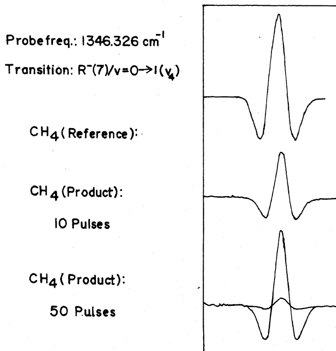
Figure 4. Growth of typical second derivative signal for \text{CH}_4 with continuing photolysis of pyruvic acid.
