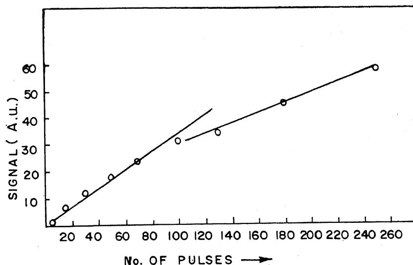
Figure 5. Growth of methane signal with number of excimer laser pulses. In the beginning the signal grows at a faster rate but eventually slows down after about 100 pulses.
