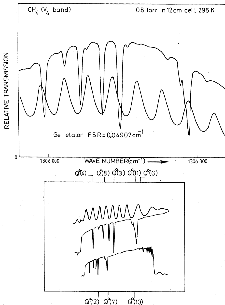
Figure 1. Typical single mode of the diode laser ( T = 80 K, I = 0.562 A) scanning the band-centre at 1306 \text{cm}^{-1} . Several Q^{(0)} lines are indicated (0.1 Torr \text{CH}_4 , 30 cm cell). This can be compared with the upper figure taken from Restelli and Cappellani (1979).
