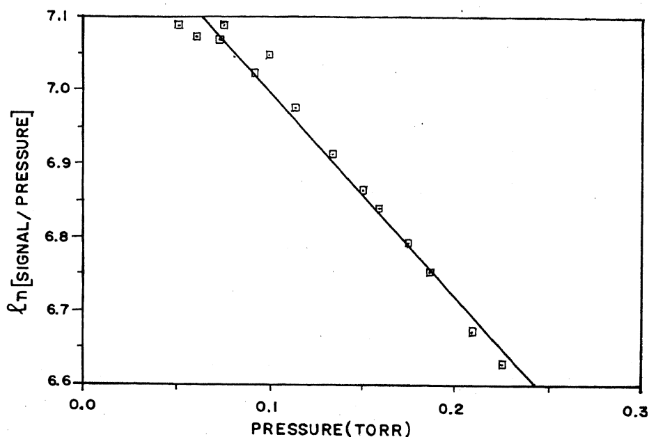
Figure 2. Calibration curve for methane using second-derivative spectroscopy. The signal is measured from negative to positive excursion. The solid line is least-square fit to the data.
