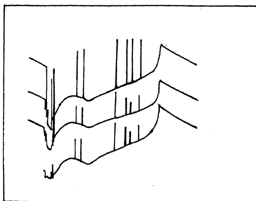
Figure 3. Digital oscilloscope recordings for methane transitions around 1346.326\text{ cm}^{-1} under full modulation amplitude ( \sim 2\text{ cm}^{-1} scan). Top and bottom traces are for 1.0 and 0.1 Torr \text{CH}_4 respectively. Middle trace is for \text{CH}_4 produced in photolysis of pyruvic acid with 400 excimer laser pulses.
