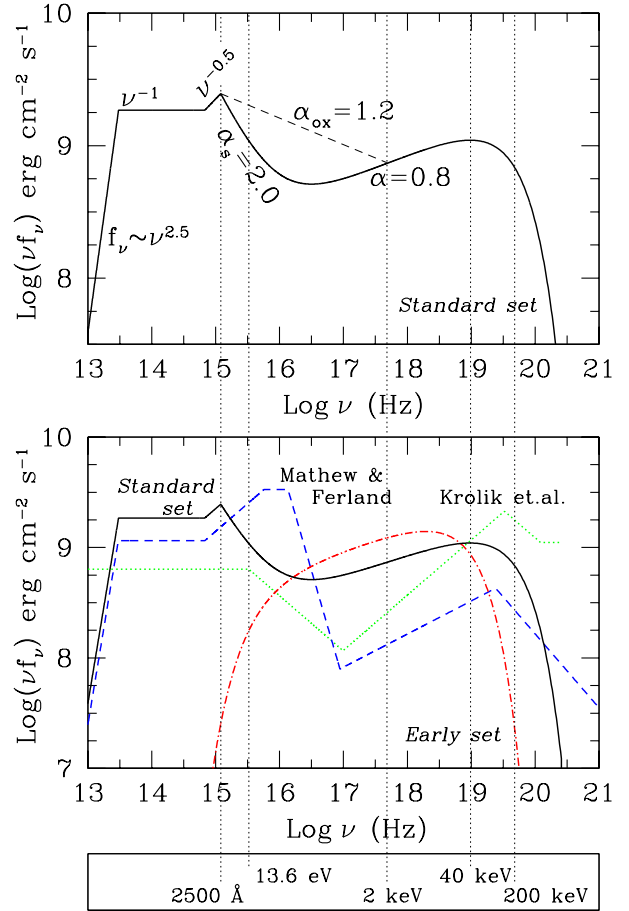
Figure 1. Top panel : Ionizing continuum obtained using Equation 6 and Equation 7 taken together, where \alpha = 0.8 , \alpha_s = 2.0 , \alpha_{ox} = 1.2 and the continuum is exponentially cut-off at 200 \text{ keV} . At lower energies, this continuum is cut-off following Equation 7 with the successive spectral indices of -0.5 , -1.0 and 2.5 . This continuum is labeled as the Standard set . We have also appropriately labeled the dominant component of the SED at various energies and used the dashed line to show the resultant \alpha_{ox} = 1.2 . Bottom panel : Comparison of the Standard set ionizing continuum with various other SEDs used or discussed in this paper. The dotted-and-dashed line labeled as the Early set is the ionizing continuum given by Equation 4 with a X-ray slope \alpha = 0.8 and exponential cut-offs at E_{min} = 13.6 \text{ eV} and E_{max} = 40 \text{ keV} . The dotted line represents the ionizing continuum used by Krolik et al. 1981 and the dashed line that used by Mathew & Ferland (1987). The important energy values including the upper and lower energy cut-offs ( 13.6 \text{ eV} , 40 \text{ keV} and 200 \text{ keV} ) and the range of definition for \alpha_{ox} ( 2500\text{\AA} and 2 \text{ keV} ) have been marked and labeled.
