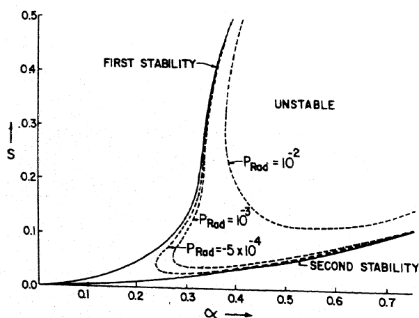
Figure 8. Marginal stability curves for ideal ballooning modes in s - \alpha plane ( s is shear parameter and \alpha is pressure gradient parameter). The solid curves are for P_{\text{rod}}=0 and the dashed curves are in the presence of RF waves.
