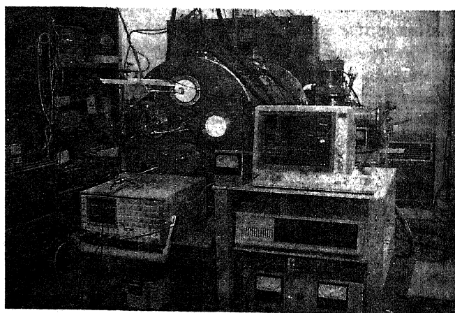
Figure 2. A view of the Double-Plasma device.
