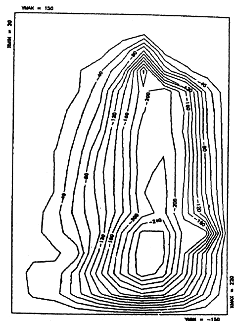
Figure 7. Contours of equipotentials (values in volts) of the electron plasma cloud obtained in non-neutral plasma device at 800 microseconds after injection. The x_{\min} and x_{\max} correspond to the inner and outer radii of vacuum vessel in mm. The toroidal field was 150 Gauss.
