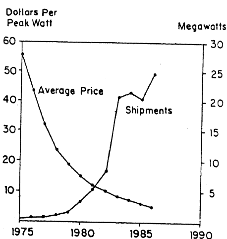
Figure 2. World photovoltaic shipments and average market prices, 1975-86. (Sources: Battelle Institute and Paul Maycode Strategies Unlimited.)
