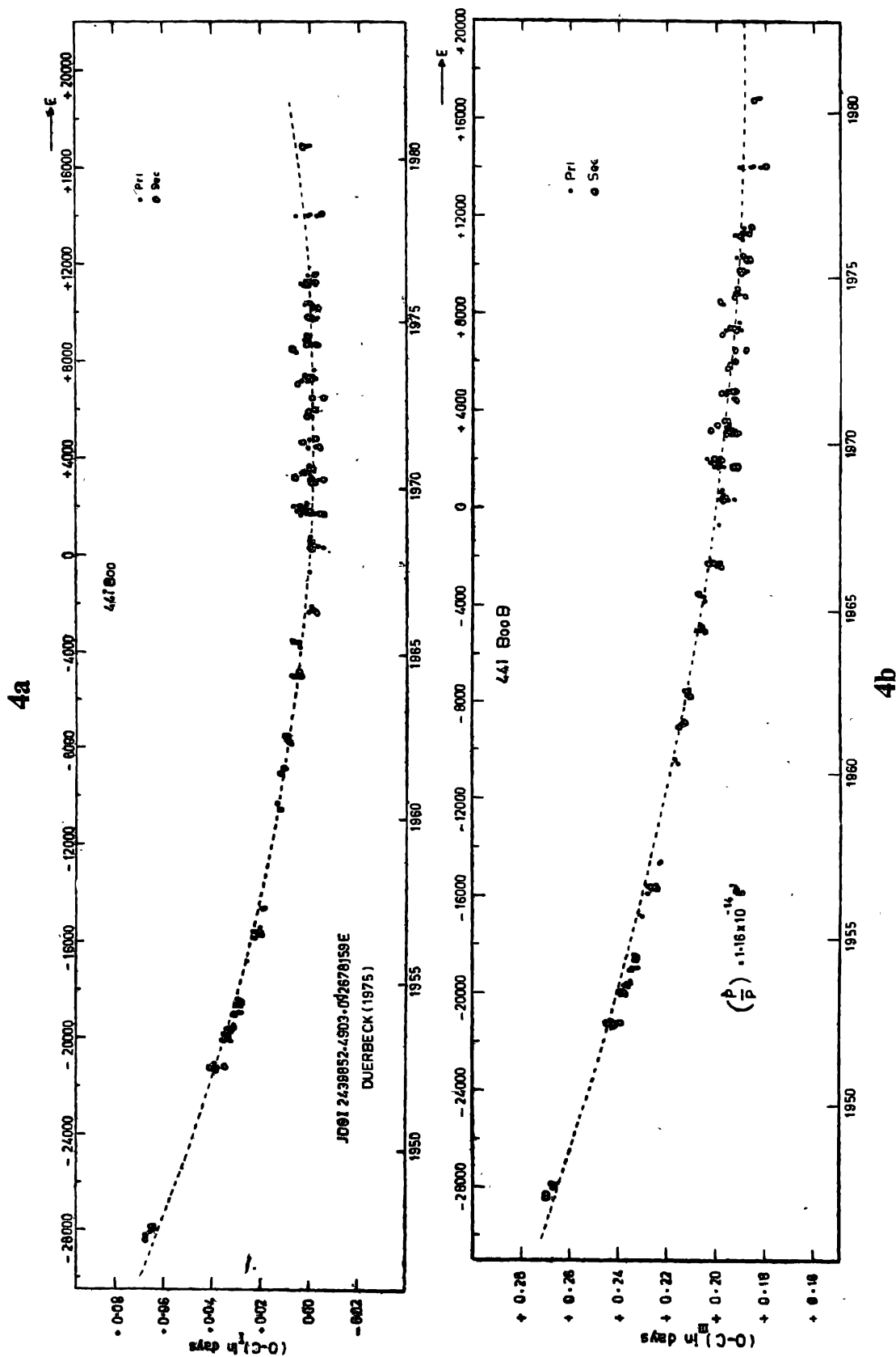
Figure 4(a). (O — C) diagram for 44i Boo B.
