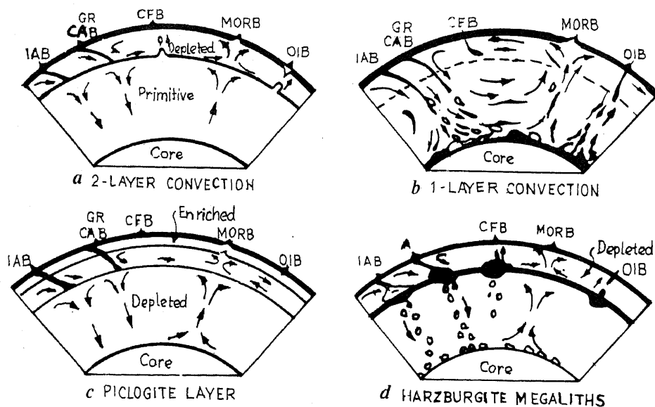
Figure 6. Convective cycles in the mantle as proposed by different workers (after Wyllie 31 ) (for explanation, see text). IAB – Island arc basalt; GR/CAB – Granite/calc-alkalic basalt; CFB – Continental flood basalt; MORB – Mid oceanic ridge basalt; OIB – Ocean island basalt.
