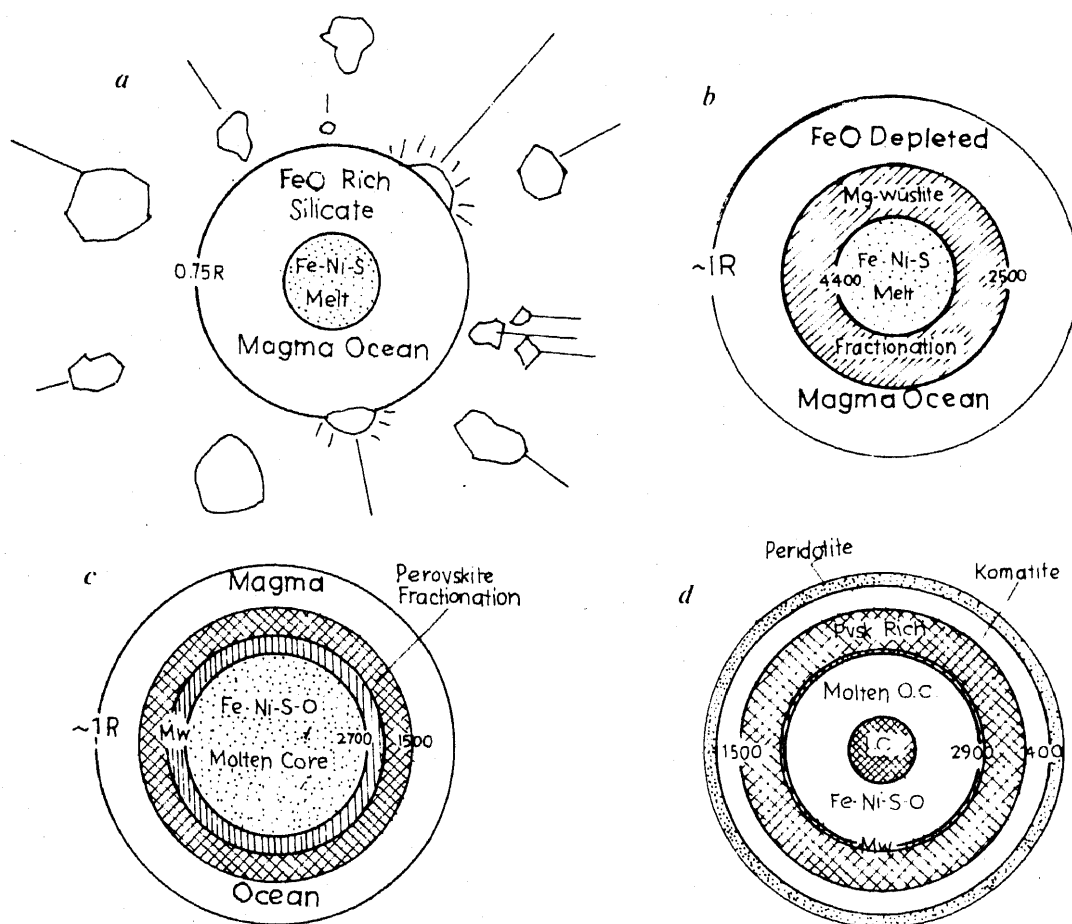
Figure 3a-d. a , Segregation of Fe-Ni-S protocore. Agee used elemental abundances of Alende meteorite to estimate the volume proportion of the silicate and Fe-Ni-S melts. Continuous impact of new chondritic materials possibly increases the size of the earth and caused more heating with a Mars size object resulting in the formation of a moon, it might have been another source of chondritic meteorite and heat for the proto-earth (after Agee 39 ). b , Formation of Fe-Ni-S proto-core accompanied by 30% magnesiowüstite fractionation. If all the fractionated magnesiowüstite were incorporated in the core, the radius will be ~400 km larger than the present core. According to Agee, in the molten silicate mantle FeO/FeO+MgO was 0.10. Although fractionation of magnesiowüstite and FeO solution in the core is shown separately in the figure, this might have happened simultaneously (after Agee 39 ). c , Later stages of differentiation in which most of the FeO from magnesiowüstite is dissolved in the molten core. Agee considers that the predominant crystalline phase at this time is Mg-perovskite, which results in the enrichment of mantle below 700 km in SiO 2 . According to Agee the depth of perovskite accumulation occurs in a layer that contains its level of natural buoyance (~1680 km) in the silicate melt (after Agee 39 ). d , Mostly solidified mantle after magmatic differentiation. Agee thinks that formation of a liquid with bulk composition similar to komatiitic liquid results due to mass balance. Layer of komatiitic melts as well as that of crystalline phases (olivine, clinopyroxene, majorite, \beta -phase, Mg and Ca-perovskite) occupy position at different levels depending on pressure temperature condition of fractionation from the magma ocean. According to Agee with the exception of peridotite the composition of layer may not be the same as that at present (after Takahashi 25 ).
