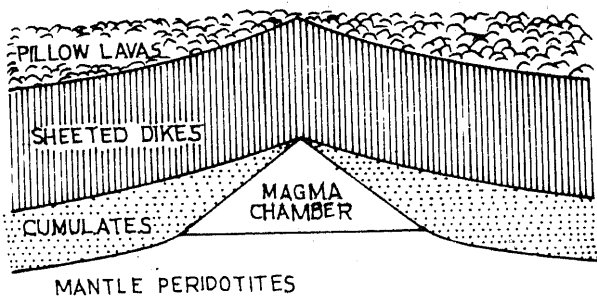
Figure 7. Illustration (not to scale) of the oceanic crust at a spreading centre (after Turcotte and Morgan 33 ).
