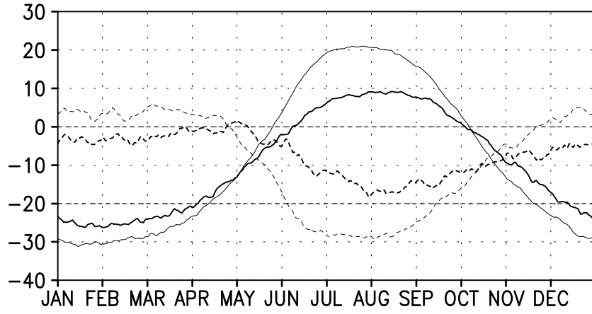
Figure 1: (Supplementary) Evolution of meridional gradient of TT between two boxes similar to those in Fig.1a but over the longitudes between 40^{\circ}\text{E} - 110^{\circ}\text{E} and 110^{\circ}\text{E} - 150^{\circ}\text{E} respectively (solid lines with increasing thickness). Zonal wind shear between 200 hPa and 850 hPa averaged between \text{Eq.}-15^{\circ}\text{N} over the two longitude domains are shown by dotted lines of respective thickness.
