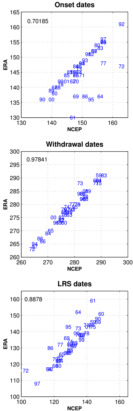
Figure 2: (Supplementary) The scatter plot of OD, WD and LRS dates from ERA and NC from 1958 to 2001. The correlation coefficient between ERA and NC are given in respective panels.
