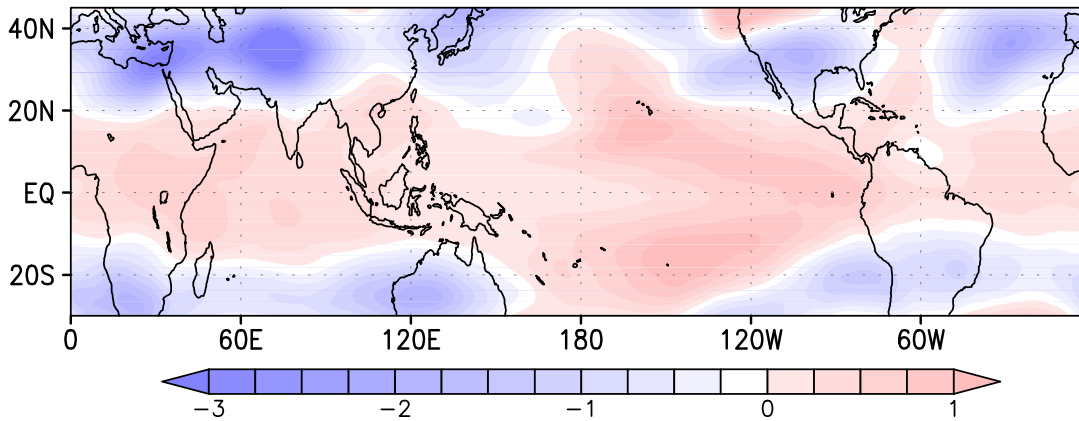
Figure 4: (Supplementary) Tropospheric temperature (TT, averaged between 200 and 700 hPa) response to El Nino SST forcing during the period between 15 May and 15 June. An ensemble of simulations of an Atmospheric General Circulation Model (AGCM, here we use NCAR CCM3) forced by El Nino composite SST were carried out. Integrations were carried out over an entire year (year(0)) of El Nino composites. Another 10 member control simulation is done with climatological SST forcing. The difference of TT between the El Nino composite run and the control run, averaged between 15 May and 15 June is plotted (K).
