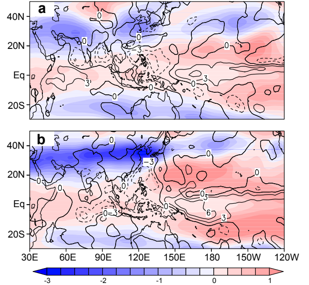
Figure 4. El Niño minus La Niña composites of TT (shaded, K) and rainfall (contours, \text{mm day}^{-1} ) anomalies averaged between (a) 15 May and 15 June and (b) 15 September and 15 October. Composites are based on 8 El Niño years (1957,65,72,79,82,87,92 and 97) and 7 La Niña years (1955,64,70,73,75,88 and 99) defined using normalized Niño4 SST anomalies being > 1 ( < -1 ).
