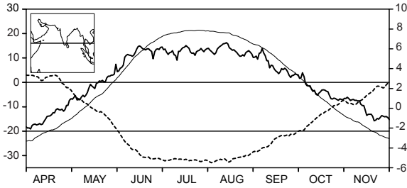
Figure 1. \Delta\text{TT} between the two boxes (thin solid, \text{K} \times 6 , the zonal extent of both boxes is between 30^\circ - 110^\circ\text{E} while the meridional extent of the northern (southern) box is between 10^\circ\text{N} - 35^\circ\text{N} ( 15^\circ\text{S} - 10^\circ\text{N} ), shown in inset), vertical shear of zonal wind (200 hPa - 850 hPa) averaged over 50^\circ\text{E} - 90^\circ\text{E} , Eq.- 15^\circ\text{N} (dashed, \text{m s}^{-1} ) and latitude of zero absolute vorticity averaged between 50^\circ\text{E} and 100^\circ\text{E} (thick solid, right scale).
