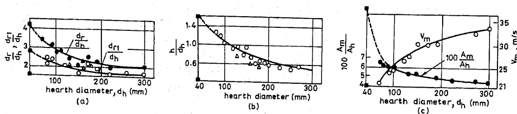
Figure 5. a. Recommended values of nozzle ring dia d_r and nozzle opening circle dia d_{r1} . The solid square ring refers to prototype parameters. b. Recommended values of h , height of the nozzle plane above hearth constriction. c. Hasselman recommendation for total nozzle area A_m .
