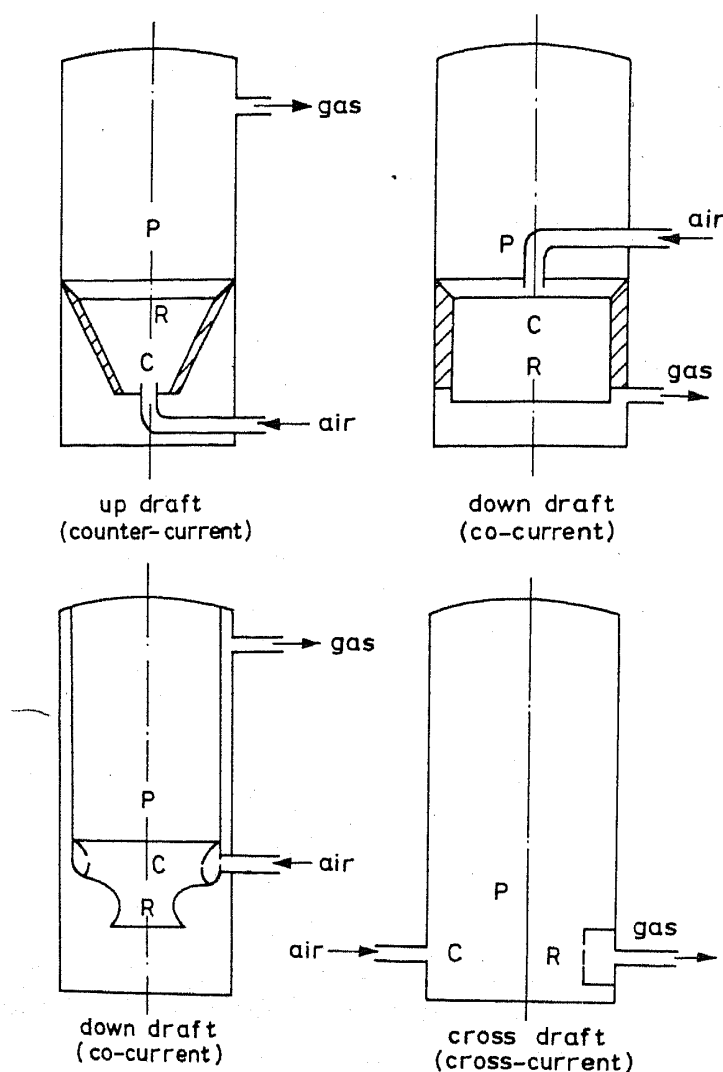
Figure 2. Reactor configurations.
