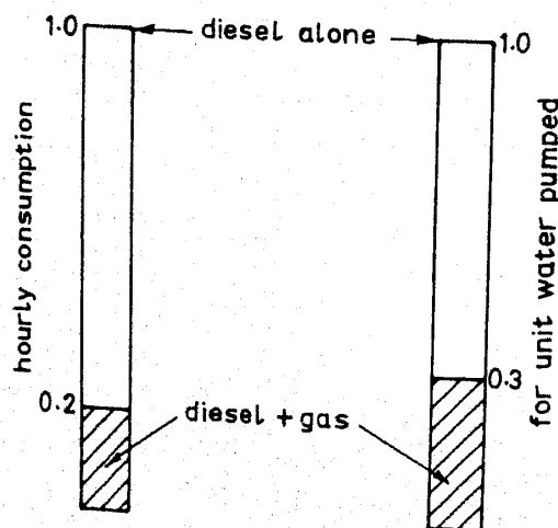
Figure 11. Diesel requirement
