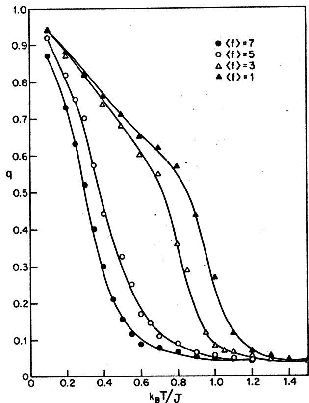
FIG. 3. The Edwards-Anderson order parameter q as a function of temperature ( k_B T/J ) for different values of \langle f \rangle . The solid lines are guides to the eye.
