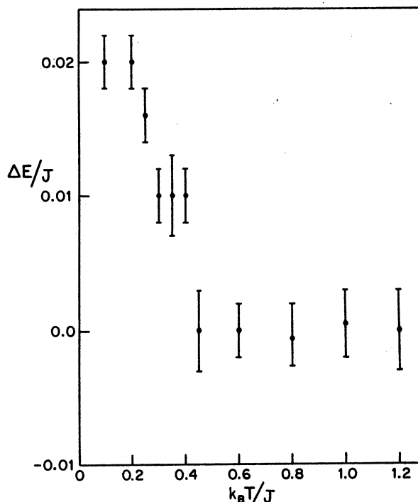
FIG. 4. Temperature dependence of \Delta E/J , the difference in energy per spin between zero-field-cooled and field-cooled runs for \langle f \rangle = 7 .
