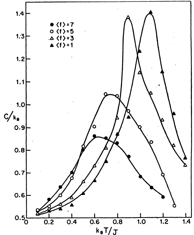
FIG. 1. The temperature (in units of J/k_B ) dependence of the specific heat per spin, C/k_B , for different values of \langle f \rangle . The solid lines are guides to the eye.
