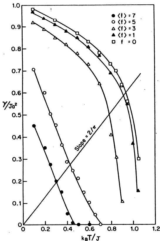
FIG. 2. The helicity modulus \gamma/Ja^2 vs the temperature k_B T/J for different values of \langle f \rangle . The solid curves are guides to the eye. The straight line of slope 2/\pi represents the universal jump in \gamma/T at the Kosterlitz-Thouless transition for f = 0 .
