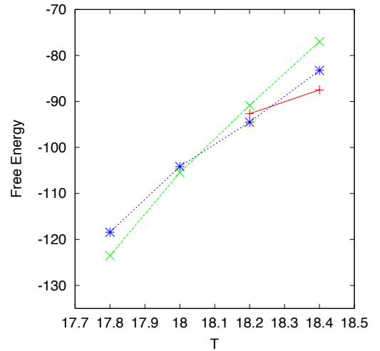
FIG. 8: (Color online). Temperature dependence of the dimensionless free energies of different local minima of a sample with N_v = 4096 and N_p = 64 (the sample is the same as the one for which results are shown in Figs. 1, 3, 4 and 7). The data for the BrG, BoG and IL minima are shown by the (green) crosses and dashed line, (blue) asterisks and dotted line and the (red) plus signs and solid line, respectively. The lines are guides to the eye.
