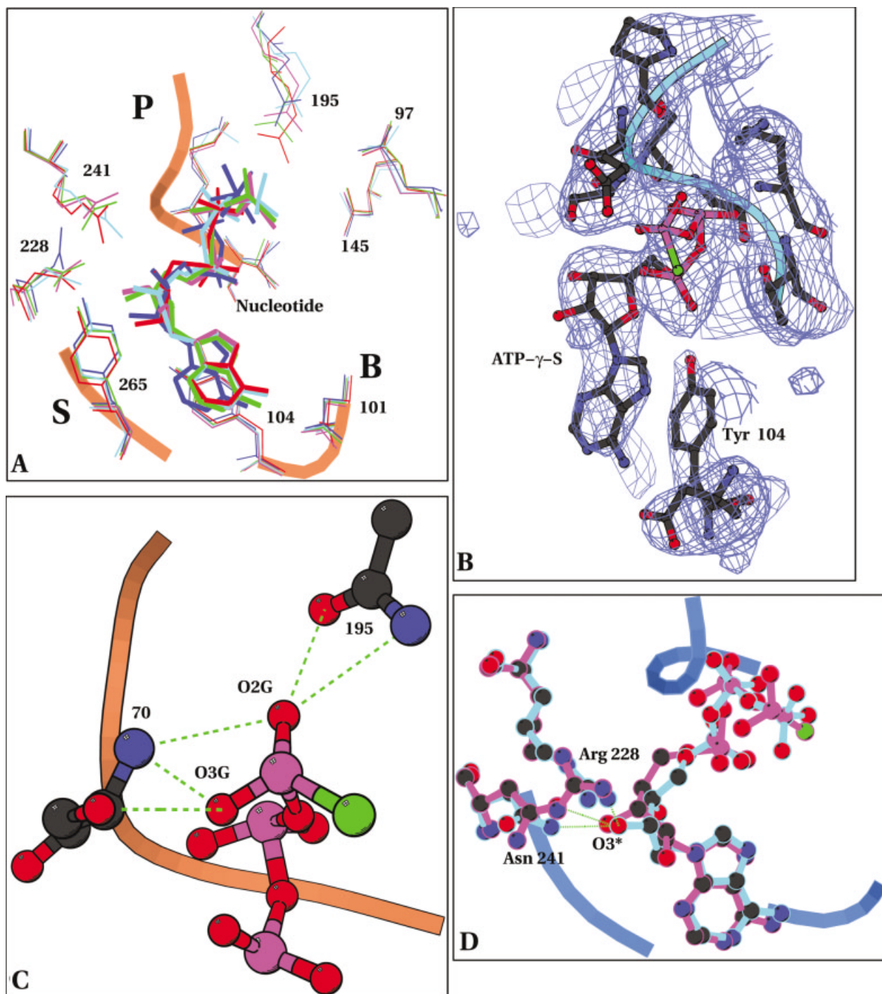
Fig. 3. A : Superposition of the nucleotide binding sites of different MtRecA complexes. The P, B, and S regions refer to the residues that bind to phosphate, base, and sugar, respectively. Residues and the nucleotide in the ADP bound structure are shown in red while those in the dATP complex are shown in cyan and those in the ATP- \gamma S complexes in the presence and absence of magnesium are shown in magenta and green, respectively. Those in the ADP- \text{AlF}_4 complex are shown in blue. This figure has been prepared using MOLSCRIPT. 38 B : An Fo-Fc omit map (contoured at 2.5 \sigma ) of the nucleotide binding site in the MtRecA-ATP- \gamma S complex. Stacking interaction of the Tyr-104 is clearly seen. The position of the P-loop is represented by a cyan ribbon. The figure has been prepared using BOBSCRIPT. 39 C : Interaction of the terminal phosphate of ATP- \gamma S with the protein. Hydrogen bonds are indicated by green dotted lines. D : Superposition of ATP- \gamma S (magenta) and dATP (cyan) complexes of MtRecA. Nucleotides and residues Arg 228 and Asn 241 are shown in ball-and-stick representation. The O3' sugar hydroxyl in dATP structure superposes on the O2' sugar hydroxyl of ATP- \gamma S.
