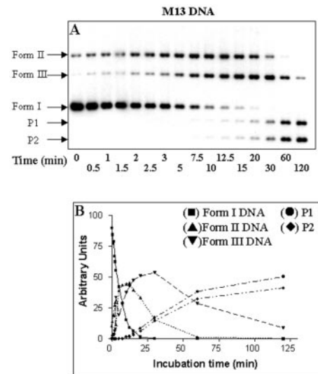
FIG. 4. Kinetics of cleavage of ectopic DNA by PI-MtuI. Reactions were performed using form I DNA (16 \mu\text{M} ) and PI-MtuI (1 \mu\text{M} ) in the presence of 5 mM \text{Mg}^{2+} . Panel A, at specified time intervals as indicated below each lane aliquots were removed, and the reaction was stopped immediately by the addition of SDS and proteinase K, followed by incubation for 15 min at 37 ^{\circ}\text{C} . The products were analyzed on an agarose gel as described in the legend to Fig. 1. The positions of substrates and products are indicated on the left. Panel B, the amount of products generated during the reaction were determined by quantification of the gel shown in A. The bands were quantified by scanning in a UVI-Tech gel documentation station using UVI-BandMap software version 99 and plotted using Graphpad Prism version 2.0. The extent of the formation of products (in arbitrary units) was plotted versus incubation time. The final cleavage products are labeled as P1 and P2. Quantification of the product generated as a function of time is an average of three independent experiments.
