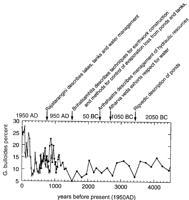
Figure 1. Monsoon winds reconstructed for the past 4500 years using per cent fossil Globigerina bulloides in Arabian Sea Box core RC 2730 (open circle) 16 and ODP 723 (solid circle) 17 . Weak summer monsoon winds are indicated by low abundances of the plankton G. bulloides in the Arabian Sea. Arid episodes correlate well with ancient Indian texts composed during those times containing descriptions of earthworks that may document aridity prevailing then: Rigveda (BC 1500, although dating of text is still unresolved), Atharva Veda (BC 800), Kautilya’s Arthashastra (BC 300), Varahamihira’s Brihatsamhita (AD 550), Kalhana’s Rajatarangini (AD 1148–1150).
