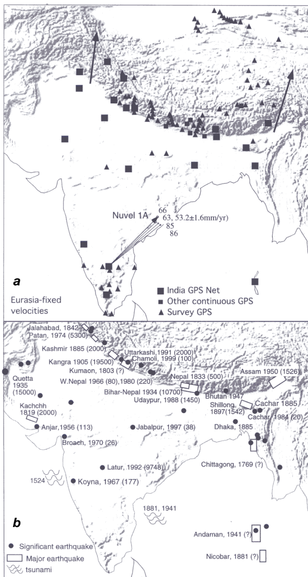
Figure 1. a, GPS measurements in India and Tibet (excluding unpublished Survey of India studies). Existing survey type measurements are indicated with triangles and planned and existing continuous tracking sites by squares. The arrows indicate NUVEL-1A velocity vectors relative to Eurasia, and show four recent estimates of the velocity of IISc, Bangalore 63,66,85,86 . (Uncertainty ellipses are less than 3% of the signal and are almost invisible at the scale shown.); b, Significant earthquakes in India with year of occurrence and fatality count known. Recently revised magnitudes for the Kangra 1905 and Shillong 1897 earthquakes 87,88 have reduced their inferred rupture-areas, leaving large segments of the Himalayan arc unruptured.
