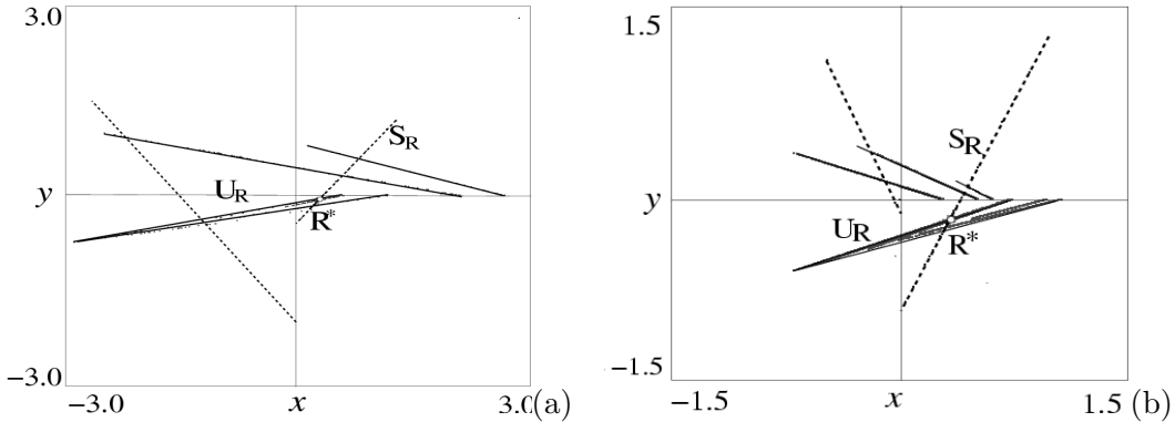
Fig. 15. (a) Homoclinic intersections of stable and unstable manifolds of the flip saddle R^* for a negative discontinuity, with \tau_L = 1.0 , \tau_R = -1.0 , \delta_L = \delta_R = 0.3 , l = -1 , \mu = 0.5 . (b) Homoclinic intersections of stable and unstable manifolds of the flip saddle R^* for a positive discontinuity, with \tau_L = 1.2 , \tau_R = -1.5 , \delta_L = \delta_R = 0.3 , l = 1 , \mu = 0.5 .
