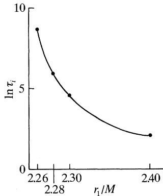
Figure 2. The damping time \tau_i (in the unit 1/M ) of the lowest quasi-stationary state as a function of r_1/M . (No stable star can have a radius r_1 \leq 2.25M .)
