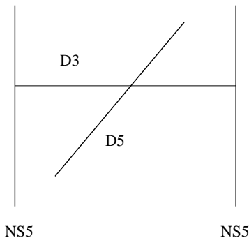
Fig.(5.1): Hanany-Witten configuration.
