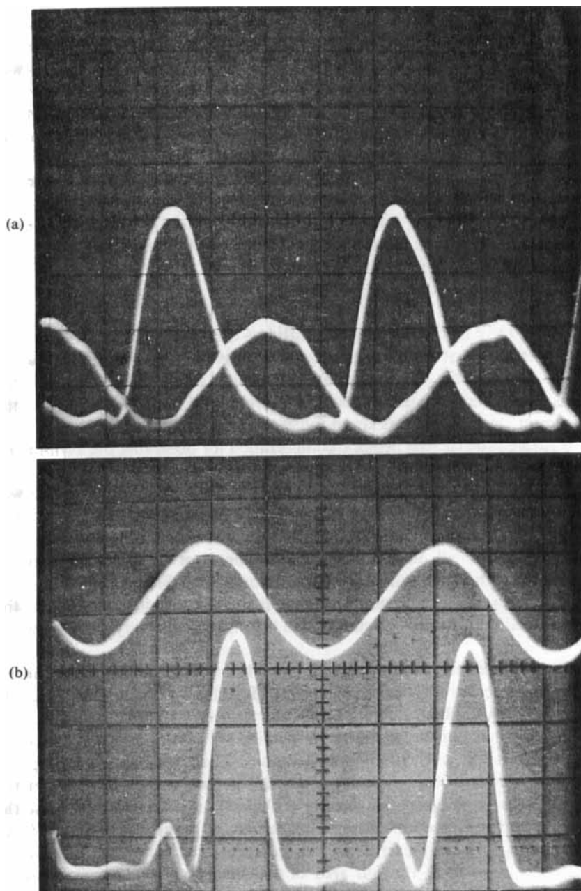
FIGURE 4 Electrooptic response as seen on an oscilloscope in the case of 20 Hz sine-wave excitation of a cell containing E7. One of the electrodes was coated with SiO and other was rubbed. Thickness \sim 12 \mu . The zero level for the electrooptic response is the bottom most line. The applied sine-wave voltage is also shown. (a) RMS voltage, 6 V; (b) RMS voltage, 10 V.
