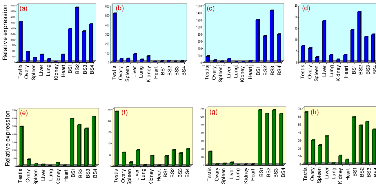
Figure 4 Quantitative expression of representative GACA/GATA-tagged transcripts demonstrating variations among somatic/gonadal tissues and spermatozoa. Four types of expressional profiles were uncovered with GACA; some transcripts with highest expression in testis and spermatozoa e.g. Ankyrin repeat domain (a), few in testis only e.g. Ubp1 (b), few in spermatozoa only e.g. novel pJSC3 (c), and others distributed almost uniformly in all the tissues e.g. HBGF-I (d). Three types of expressional profiles were observed for GATA-tagged transcripts; some showed highest expression both in testis and spermatozoa e.g. novel pJSC34 (e), few in testis only e.g. novel pJSC33 (f), few others in spermatozoa only e.g. novel pJSC32 (g), and others highest in testis and spermatozoa but with minimal variation in comparison to somatic tissues e.g. novel pJSC31 (h). For details, see table 3 and text.
