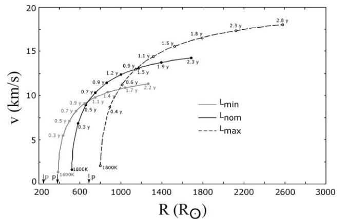
FIG. 7.—Outflow velocity as a function of radius for a CV star with mass M = 1.25 M_{\odot} , T_{\text{eff}} = 2510 K, nominal luminosity (solid curve) L_{\text{nom}} = 5080 L_{\odot} , and nominal radius R_{\text{nom}} = 377 R_{\odot} . Circles on curves are markers for 100 K decrements in grain temperature to 1000 K, starting at 1800 K. Times (in years) elapsed from 1800 K are shown next to these temperature markers. The power index k = 2.5 (optically thick outflow) in eq. (7) was used in calculating v(R) . Velocity profiles for L_{\text{min}} = 0.56L_{\text{nom}} and for L_{\text{max}} = 2.35L_{\text{nom}} are also shown. It is assumed that for L_{\text{min}} , T = T_{\text{eff}} + 200 K, and that for L_{\text{max}} , T = T_{\text{eff}} - 200 K. The arrows marked with a “P” show the position of the photosphere for the different luminosities. See text for discussion.
