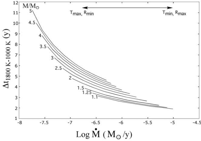
FIG. 6.—Maximum graphite growth intervals in AGB carbon star atmospheres in the temperature range T = 1800\text{--}1000\text{ K} , as a function of stellar mass and mass-loss rate. For a given stellar mass, the left end of the curve corresponds to the maximum effective temperature (3350 K) and minimum photospheric radius shown in Fig. 3, and the right end corresponds to the minimum effective temperature (2240 K) and maximum photospheric radius in that figure. The power index k = 2.5 (optically thick outflow) in eq. (7) was used. See text for discussion.
