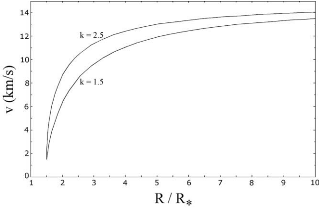
FIG. 5.—Mass outflow velocity v(R) as a function of radius R from eq. (7), for the case in which the terminal velocity v_e = 15 \text{ km s}^{-1} , R_{\text{cond}}/R_* = 1.5 , and \epsilon = 0.1 . The velocity field is shown for optically thin ( k = 1.5 ) and for optically thick outflows ( k = 2.5 ). See text for discussion.
