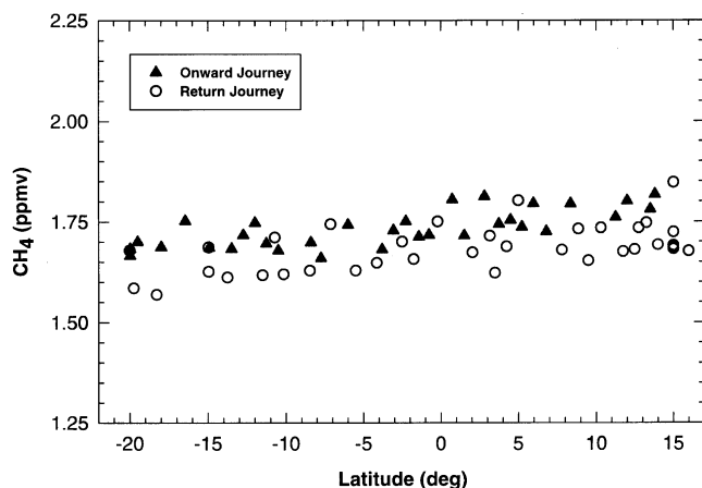
Figure 3. Latitudinal variation of CH 4 during the INDOEX IFP-1999 cruise during onward and return journeys.
