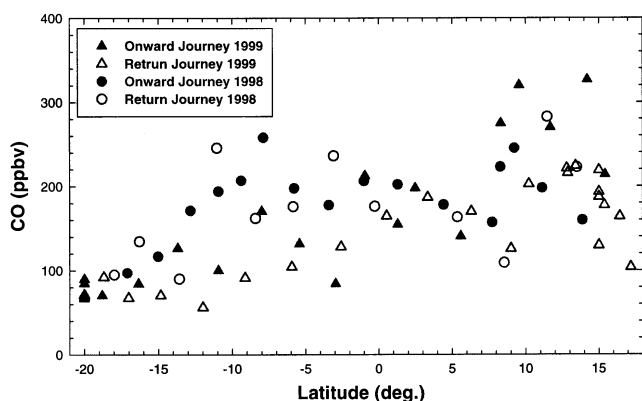
Figure 2. Latitudinal variations of daily average CO during onward and return journeys of INDOEX FFP-1998 and INDOEX IFP-1999 cruises.
