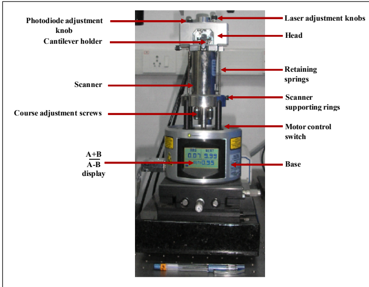
Figure 2. A modern AFM.
