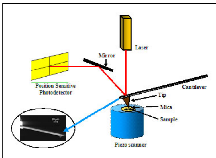
Figure 3. Mode of action of an AFM: AFM consists of an extremely sharp tip (brown color) mounted or integrated at the end of a tiny cantilever spring which is moved by a mechanical scanner/Piezo scanner (blue color) over the surface to be observed/ scanned. A magnified image of a real cantilever is also shown.
