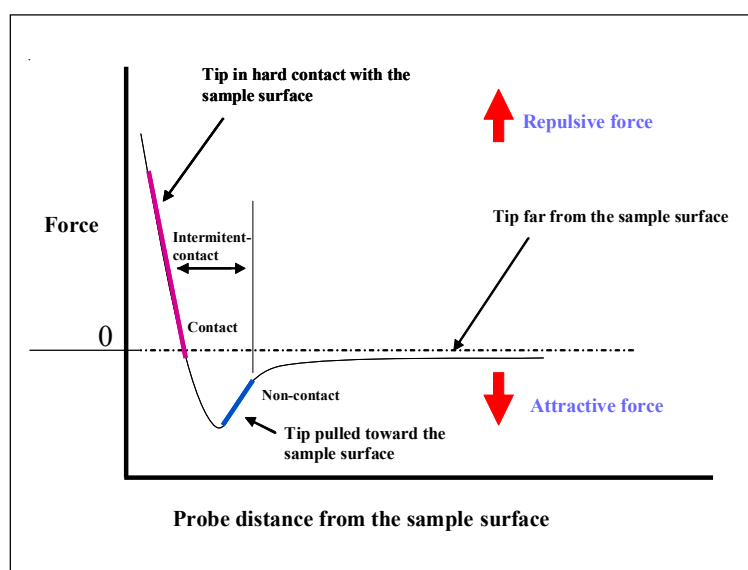
Figure 4. Graphical representation of force–distance relationship: The Y-axis of the curve represents the interatomic force acting between the cantilever and the sample surface, while the X-axis represents the distance between the cantilever and the sample surface. In the contact zone of the curve, a repulsive interatomic force mainly prevails between the cantilever and the sample where the cantilever is held a few angstroms from the sample surface. Here the AFM tip makes soft ‘physical contact’ with the sample. In the non-contact zone, the cantilever is held away from the sample surface and an attractive interatomic force prevails.
