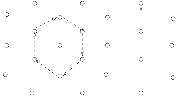
FIG. 1. A schematic diagram of cooperative ring exchange events on a ring and line. The vortices are indicated by the small circles.
