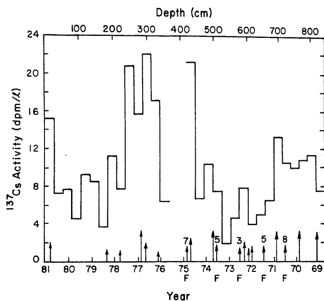
Figure 1. Variation of ^{137}\text{Cs} activity with depth of ice. Tests conducted by France are designated by F and the total number of explosions in a year are indicated above the arrows.
