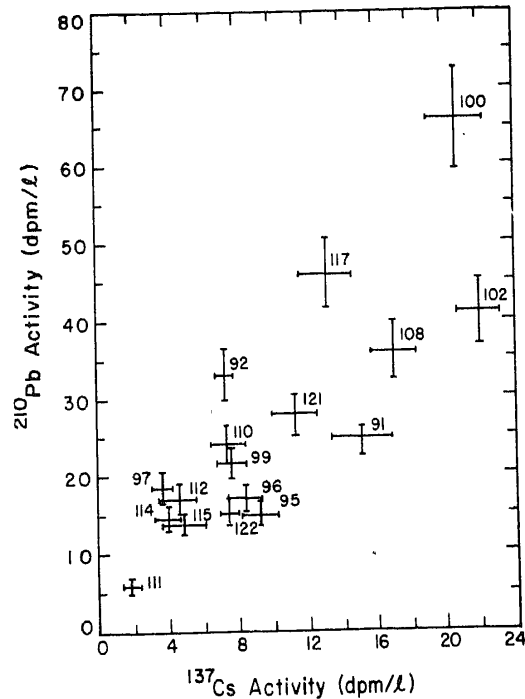
Figure 2. Variation of ^{210}\text{Pb} and ^{137}\text{Cs} activity in ice samples. Numbers refer to the CK samples as given in table 1.
