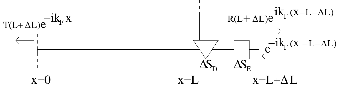
FIG. 1: Shows disordered sample of length L embedded invariantly in a supersample of length L + \Delta L . Shown also are the elementary matrices for the elastic ( \Delta S_E ) and the decohering ( \Delta S_D ) scatterings in \Delta L , with the incident, the transmitted, and the reflected waves at Fermi wavevector k_F .
