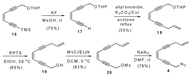
Scheme 4 Synthesis of 4.
