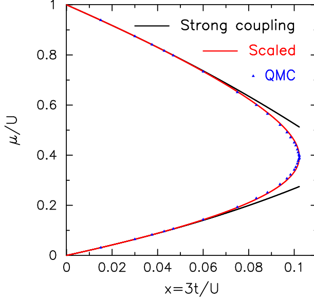
FIG. 9: (Color online) Phase diagram of the three-dimensional Bose Hubbard model. Note how the truncated strong-coupling expansion does not agree so well with the QMC data [17], but the scaled results nearly fit the Mott phase lobe perfectly.
