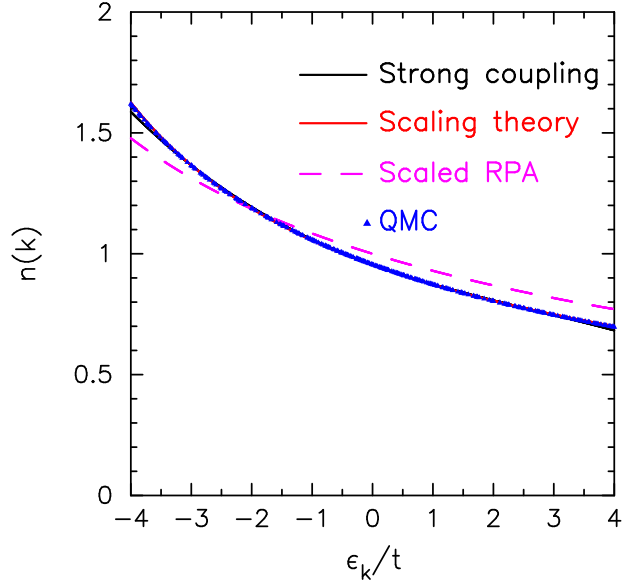
FIG. 10: (Color online) Momentum distribution function in two dimensions with x = 0.05 . We plot the strong-coupling expansion against the scaling theory results, the scaled RPA, and QMC simulations. Note how the QMC results agree much better with the scaled results and do not show the change in curvature near \xi_{\mathbf{k}} = 1 . In addition, the scaled RPA doesn't work as well here as it did in three dimensions.
