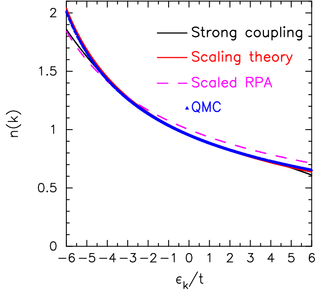
FIG. 7: (Color online) Momentum distribution function for the three-dimensional case with x = 0.0625 as a function of the band energy \epsilon_{\mathbf{k}} . Note how the QMC data agrees better with the scaling theory results than it does with the strong-coupling results or the scaled RPA, although deviations can be seen in the data.
