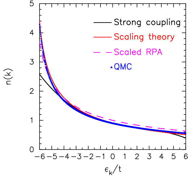
FIG. 8: (Color online) Momentum distribution function for the three-dimensional case with x = 0.09 as a function of the band energy \epsilon_{\mathbf{k}} . Once again, the QMC data agrees better with the scaling theory than it does with the strong-coupling results or the scaled RPA, although deviations can still be seen in the data. Note that the scaled RPA works better than the truncated strong-coupling expansion.
