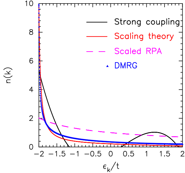
FIG. 14: (Color online) Momentum distribution function in one dimension with x = 0.2 , which is two-thirds of the way to the critical point. We plot the strong-coupling expansion against the scaling theory results, the scaled RPA, and the DMRG calculations. Note how the DMRG results agree much better with the scaling theory results than the truncated expansion or the scaled RPA, but one can see that the scaling approach is beginning to fail.
