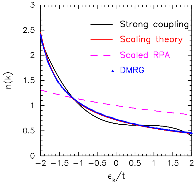
FIG. 13: (Color online) Momentum distribution function in one dimension with x = 0.1 , which is far from the critical point. We plot the strong-coupling expansion against the scaling theory results, the scaled RPA, and the DMRG calculations. Note how the DMRG results agree much better with the scaling theory results than the truncated expansion or the scaled RPA.
