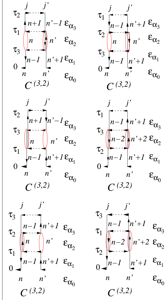
FIG. 6: (Color online.) Strong-coupling “diagrams” for the correlation functions C^{(3,2)} . The horizontal directed dashed lines indicate the hopping matrix element \mathfrak{t} between the sites labeled, and the vertical lines indicate single-site Green’s functions \mathcal{G} . The ellipses (red) at multiply visited sites denote the appearance of connected or cumulant Green’s functions. Initial and intermediate state labels for the different possible i-time orderings shown are also indicated.
