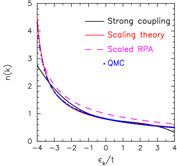
FIG. 11: (Color online) Momentum distribution function in two dimensions with x = 0.1 , which is close to the critical point. We plot the strong-coupling expansion against the scaling theory results, the scaled RPA, and the QMC simulations. Note how the QMC results agree much better with the scaling theory results.
