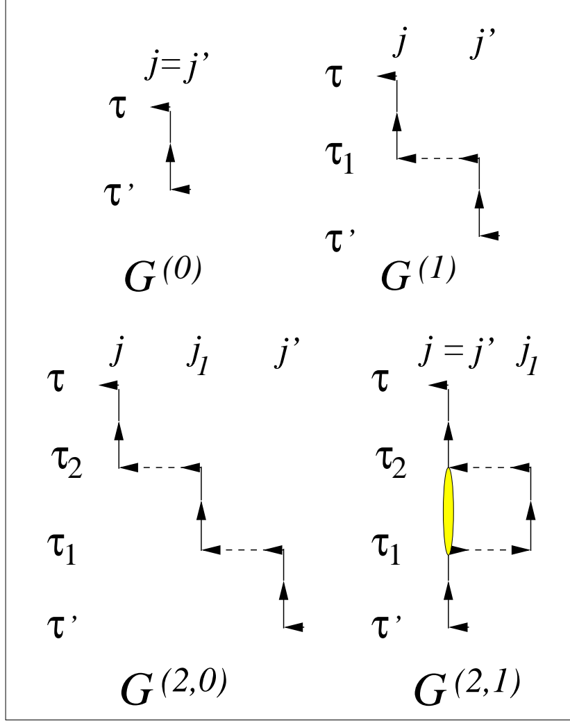
FIG. 1: (Color online.) Strong-coupling “diagrams” for the single-particle Green’s functions up to second order in t . The horizontal directed dashed lines indicate the hopping matrix element t between the sites labeled, and the vertical lines indicate single-site Green’s functions \mathcal{G} evolving between the respective i -times. The ellipses (yellow) at multiply visited sites denote the appearance of connected or cumulant n -particle Green’s functions.
