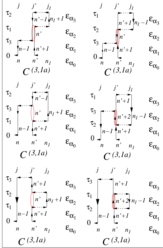
FIG. 5: (Color online.) Strong-coupling “diagrams” for the correlation functions C^{(3,1)} . The horizontal directed dashed lines indicate the hopping matrix t between the sites labeled, and the vertical lines indicate single-site Green’s functions \mathcal{G} . The ellipses (red) at multiply visited sites denote the appearance of connected or cumulant Green’s functions. Initial and intermediate state labels for the different possible i -time orderings shown are also indicated.
