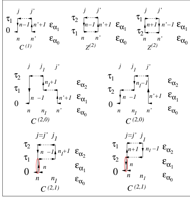
FIG. 3: Strong coupling “diagrams” for the correlation functions up to second order in \mathfrak{t} . The horizontal directed dashed lines indicate \mathfrak{t} between the sites labeled, and the vertical lines indicate single site Greens functions \mathcal{G} . The ellipses (red on line) at multiply visited sites denote the appearance of connected or cumulant Greens functions. Initial and intermediate state labels for the different possible i-time orderings shown are also indicated.
