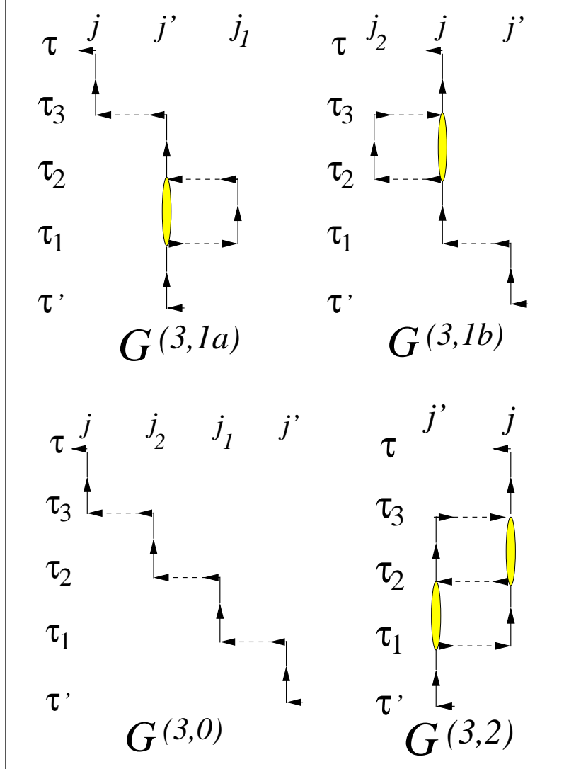
FIG. 2: (Color online.) Strong-coupling “diagrams” for the single-particle Green’s functions corresponding to third order in t . The horizontal directed dashed lines indicate the hopping matrix element t between the sites labeled, and the vertical lines indicate single-site Green’s functions \mathcal{G} evolving between the respective i -time. The ellipses (yellow) at multiply visited sites denote the appearance of connected or cumulant n -particle Green’s functions.
