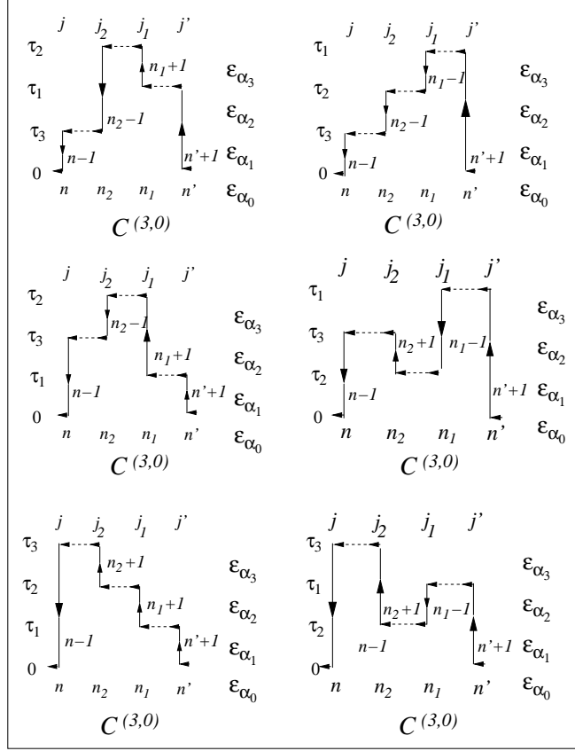
FIG. 4: (Color online.) Strong-coupling “diagrams” for the correlation functions C^{(3,0)} . The horizontal directed dashed lines indicate the hopping matrix \mathbf{t} between the sites labeled, and the vertical lines indicate single-site Green’s functions \mathcal{G} . The ellipses (red) at multiply visited sites denote the appearance of connected or cumulant Green’s functions. Initial and intermediate state labels for the different possible i -time orderings shown are also indicated.
