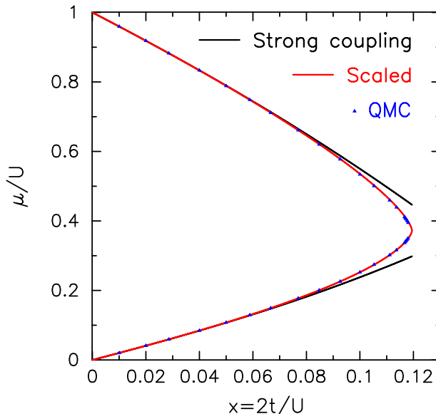
FIG. 12: (Color online) Phase diagram of the two-dimensional Bose Hubbard model. Note how the truncated strong-coupling expansion [8, 9] does not agree so well with the QMC data [16], but the scaled results nearly fit the Mott phase lobe perfectly.
