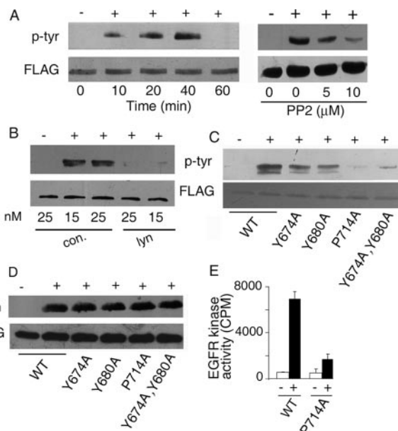
FIGURE 4. HP0175 activates Lyn-mediated TLR4 phosphorylation and EGFR kinase. A , AGS cells were transfected with wild type (WT) FLAG-tagged TLR4 or its mutants as indicated ( A–E ). A , cells transfected with WT-TLR4 were left untreated or treated with PP2 at different concentrations, followed by treatment without (–) or with (+) HP0175 for the indicated time periods ( A ) or for 40 min ( C–E ). B , cells were transfected with either control siRNA ( con. ) or Lyn siRNA ( lyn ), followed by treatment without (–) or with (+) HP0175. Cells were lysed after treatments. For A–D , lysates were immunoprecipitated with M2 FLAG-agarose, and Western blotting was performed with anti-phosphotyrosine antibody ( A–C ) or with anti-Lyn antibody ( D ). Blots were reprobed with anti-FLAG antibody to ensure equal loading. E , EGFR kinase activity was measured as described in the legend to Fig. 2A. Results in E represent the means \pm S.D. of three separate experiments. Blots are representative of three separate experiments. HP0175 was used at a concentration of 1 \mu g/ml.
