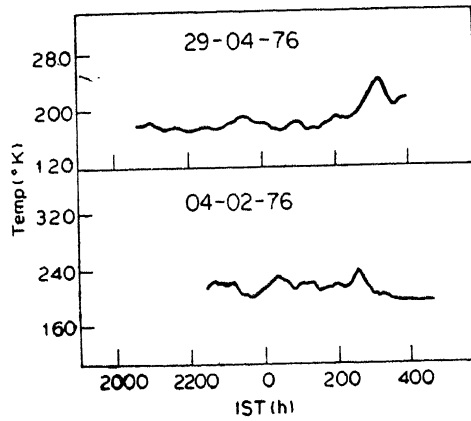
Figure 2. Short periodicity ( \approx 10 to 120 min) in temperature fluctuations during two typical nights.
