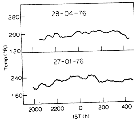
Figure 3. Short and long periodicity in temperature fluctuations during two typical nights.
