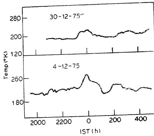
Figure 1. Long periodicity ( \approx 4 hr) in temperature fluctuations.
