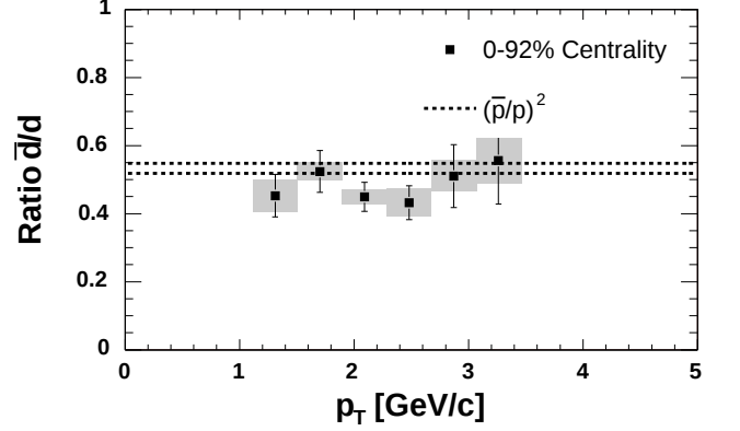
FIG. 5: \bar{d}/d ratio vs. p_T for minimum bias data. The dashed lines represent the square of the measured \bar{p}/p ratio as a function of p_T within uncertainties.
