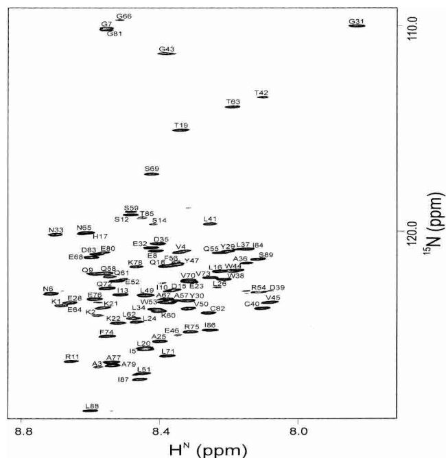
Figure 3. ^1\text{H} - ^{15}\text{N} HSQC spectrum of barstar in 8 M urea at pH 6.5 and 25°C. The ^1\text{H}^{\text{N}} and ^{15}\text{N} backbone assignments are indicated.
