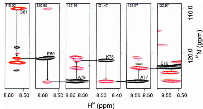
Figure 2. Illustrative sequential walk through F_1 – F_3 planes in the HNN spectrum of barstar in 8 M urea at pH 6.5 and 25°C. Sequential connectivities are indicated for the Gly 81 to Glu 76 stretch in the protein primary sequence. Strips from the spectra at the appropriate \text{H}^{\text{N}} chemical shifts are shown. Black and red contours are positive and negative peaks, respectively. The distinct Gly 81 plane in the HNN spectrum served as a starting triplet fixed point to obtain sequential connectivities. The F_2 ( ^{15}\text{N} ) chemical shift is indicated at the top of each strip of the HNN spectrum (for details, see Bhavesh et al. 2001 and Panchal et al. 2001).
