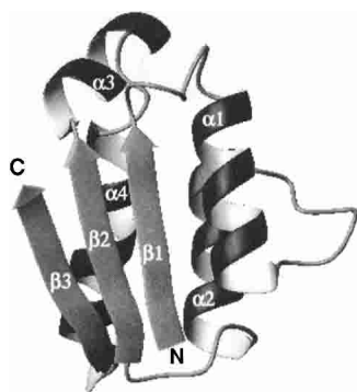
Figure 1. NMR structure of barstar (PDB ID 1BTA; Lubienski et al. 1994).
