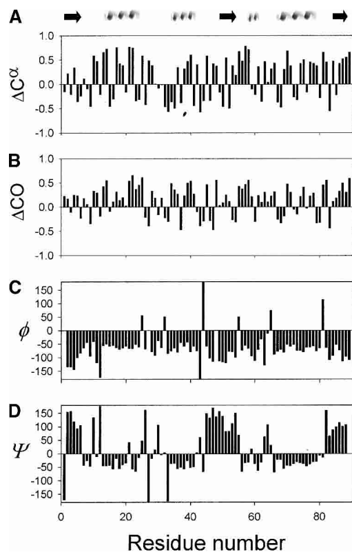
Figure 4. Secondary chemical shifts for (A) C_{\alpha} and (B) CO resonances in barstar in 8 M urea at pH 6.5 and 25°C. The chemical shifts have been corrected for contributions from the local amino acid sequence (Schwarzinger et al. 2001). Reference random coil shifts used are those determined for the peptide Ac-GGXGG-NH 2 in 8 M urea at pH 2.3 (Schwarzinger et al. 2000). The \phi , \psi backbone dihedral angles for native barstar are plotted against the primary sequence in C and D, respectively. The native secondary structural elements are indicated at the top in the figure.
