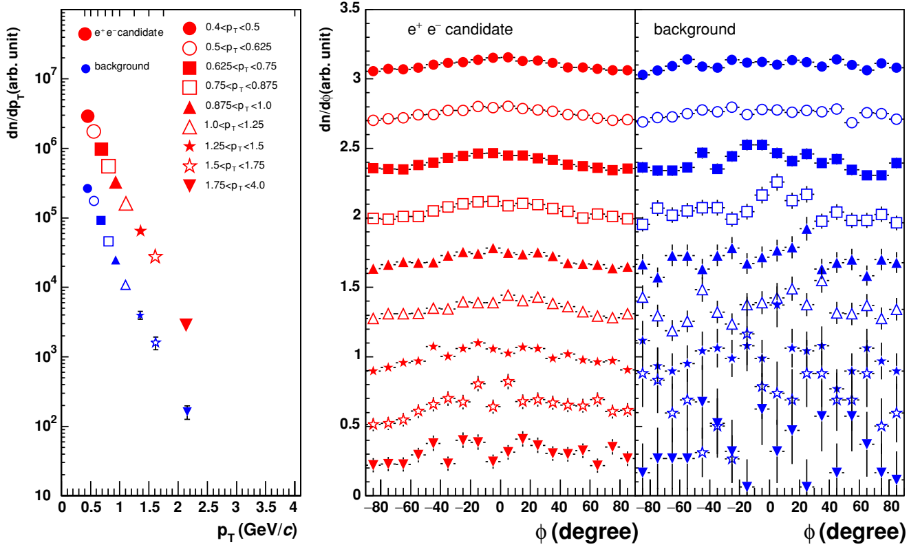
FIG. 5. (Color online) Azimuthal distributions relative to the reaction plane of electrons (middle panel) and the background (right panel) in each momentum bin. The distributions are overlaid by shifting them on the vertical axis such that the spacing between each is equal. The raw yields of each distribution are shown in the left panel.
