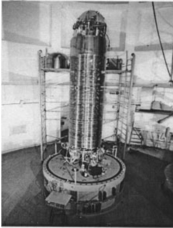
Figure 1. High voltage column section of the FOTIA. The 180^\circ -magnet and other components inside the terminal can also be seen.
