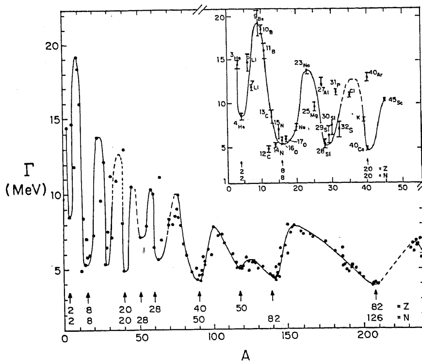
Figure 1. \Gamma is the full width at half maximum of the total photon-neutron cross section on a nucleus when plotted as a function of the incident photon energy. Compilation of the cross-section data by Dietrich and Berman [9] was used to determine \Gamma . Note the systematic modulations in the \Gamma vs A curve, with minima at the proton ( Z ) or neutron ( N ) magic numbers. The minimum at A = 28 corresponds to ^{28}\text{Si} , see [12]. The curve is drawn as a guide to the eye. Dashed lines indicate regions of sparse or nonexistent data. The inset shows the region A \leq 45 in greater detail. ( \Gamma for Ne, Cl and K is obtained from data on natural samples.) The statistical significance of the oscillations of the curve is discussed in the text.
