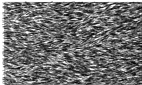
FIG. 10: A typical configuration for a 25 \times 15 -sized system with a uniform \kappa gradient, with \kappa_L = 32 and \kappa_R = 50 at the two ends respectively. The horizontal alignment induced by the gradient is evident.
