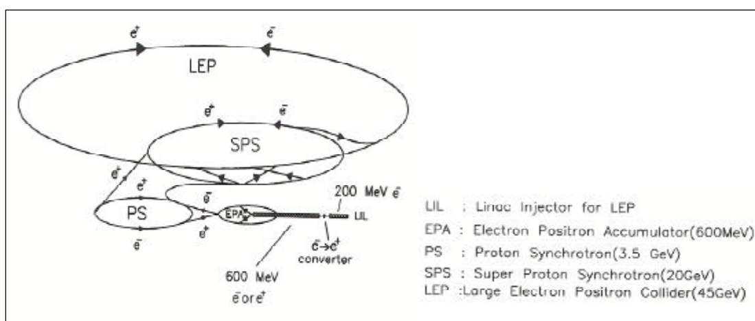
Figure 1. Acceleration of electrons and positrons for LEP.
