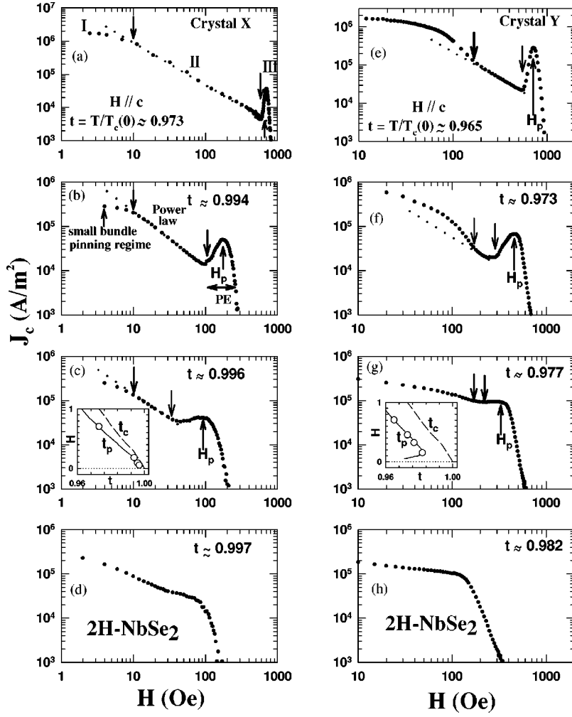
FIG. 1. Log-log plots of J_c vs H(\parallel c) at selected temperatures in crystals X and Y of 2H\text{-NbSe}_2 . The three different pinning regimes (I, II, and III) have been identified at t=0.973 in crystal X in (a). The insets in (c) and (g) display the PE curve t_p(H) [=T_p(H)/T_c(0)] and the superconductor-normal phase boundary t_c(H) [=T_c(H)/T_c(0)] in crystals X and Y, respectively (Ref. 11). The marked data points on the PE curves in each of these insets identify the reduced temperatures at which J_c(H) data have been displayed in (a)–(d) and in (e)–(h). The J_c(H) plot at t=0.997 in crystal X in (d) and that at t=0.982 in crystal Y in (h) show that the peak effect cannot be identified distinctly at the corresponding temperatures. Note the location of these two reduced temperature values in the insets of (c) and (g), respectively; they lie near the ‘nose’ region of the respective t_p(H) curves.
