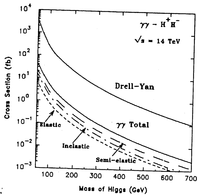
Figure 1. Cross section in fb for DY and \gamma\gamma production of the charged Higgs at LHC energies, as a function of the Higgs mass. The dashed, dash-dotted and long-dashed lines show the el., inel. and semi-el. contributions (as defined in the text) to the \gamma\gamma cross sections. The total \gamma\gamma cross section and the DY contributions are shown by the labeled solid lines.
