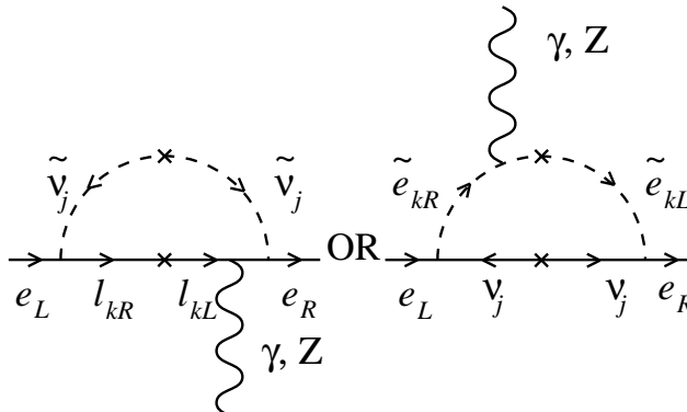
Figure 2: One loop diagrams contributing to the edm of electron in the presence of Majorana masses for the neutrinos(sneutrinos). Note that here and in all the other diagrams, the \gamma/Z is to be attached to all possible lines to which it couples.
