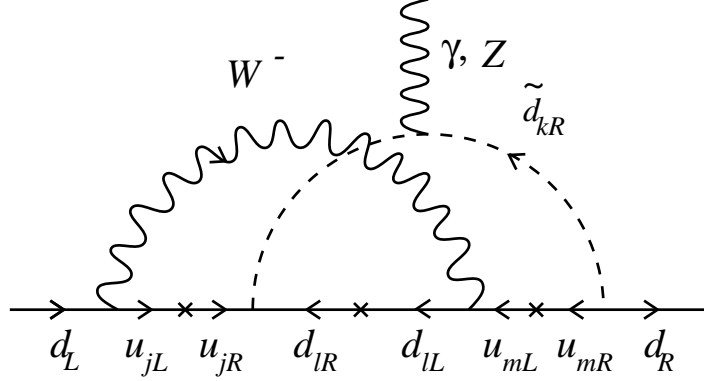
Figure 6: An example of the leading two loop contribution to the down quark edm due to \lambda'' couplings.
