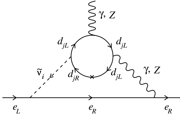
Figure 4: An example of the leading two loop contribution to the electron edm due to \lambda' and \lambda couplings.
