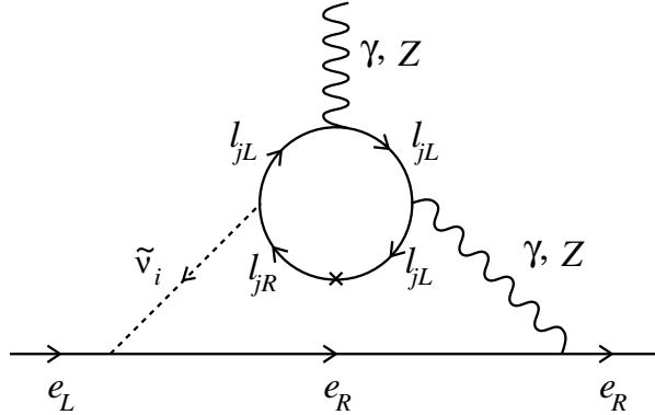
Figure 3: An example of the leading two-loop contribution to the edm of electron due to \lambda couplings.
