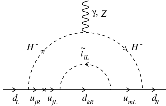
Figure 5: An example of the Higgs mediated two loop contribution to the edm of the down quark due to \lambda' couplings.
