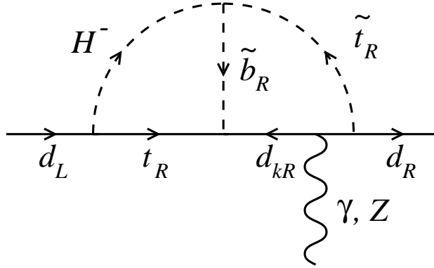
Figure 7: An example of the two loop contribution to the edm of the down quark due to \lambda'' couplings and supersymmetric interactions of the Higgs.
