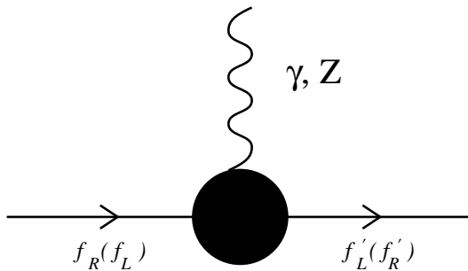
Figure 1: Generic diagram which will contribute to the dipole moment.
