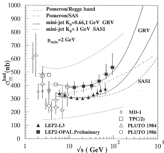
Figure 7. Total inelastic photon-photon cross-section in the eikonized mini-jet model with p_{T\text{min}} = 2 GeV, compared with data and Regge/Pomeron parametrization (see [23] for details). The two lower mini-jet curves correspond to k_0 = 1 GeV with GRV and SAS1 densities. The highest one is for GRV densities and k_0 = 0.66 GeV.
