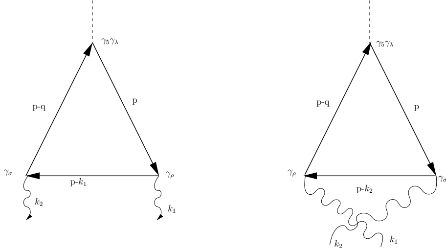
FIG. 1: The ABJ triangle diagram(left panel) and its crossed counter part(right panel).
