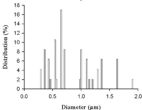
Fig 2: The particle size distribution of the microspheres
