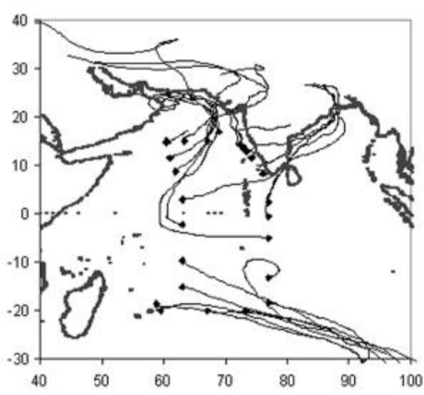
Figure 2. Air back trajectories computed by the HYSPLIT-4 model using NCEP wind data for the January to March 1999 period (courtesy: NCMRWF, New Delhi). The thin lines show the path an air parcel would have taken before reaching the ocean surface. Air parcels originating as far as Turkey (40°N, 40°E), Iran and Pakistan could find its way to the mid-Arabian Sea, while below about 8°S the wind is predominantly from the southeast direction. During the 10 days air back trajectories the air parcels were found to lie within about 1 km altitude, all along its path.
