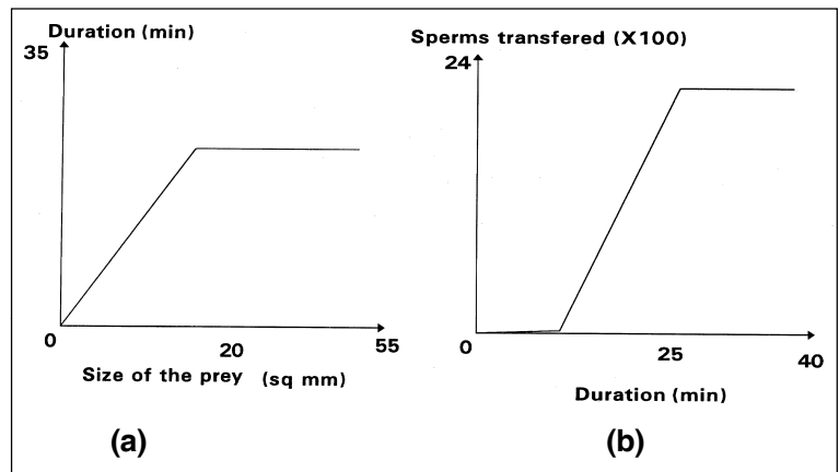
Figure 2. (a) Relation between the size of the prey presented as a nuptial gift and the duration of copulation in Black Tipped Hanging flies. (b) Relation between the duration of copulation and the number of sperms transferred in Beach Tipped Hanging flies.
