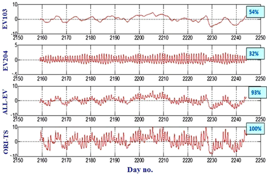
Fig. 7 Plot of decomposed eigenvector in atmospheric temperature grouped into two classes at Hsinhou from November 29, 2011 to February 22, 2012
